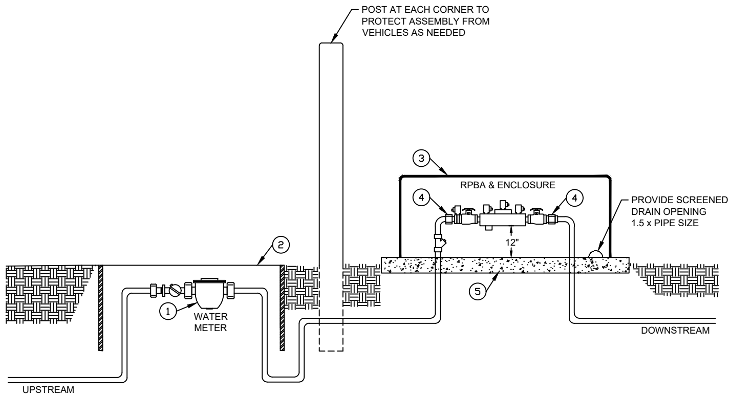
RPBA ASSEMBLY
