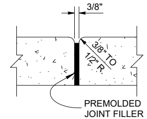
(E) EXPANSION JOINT
