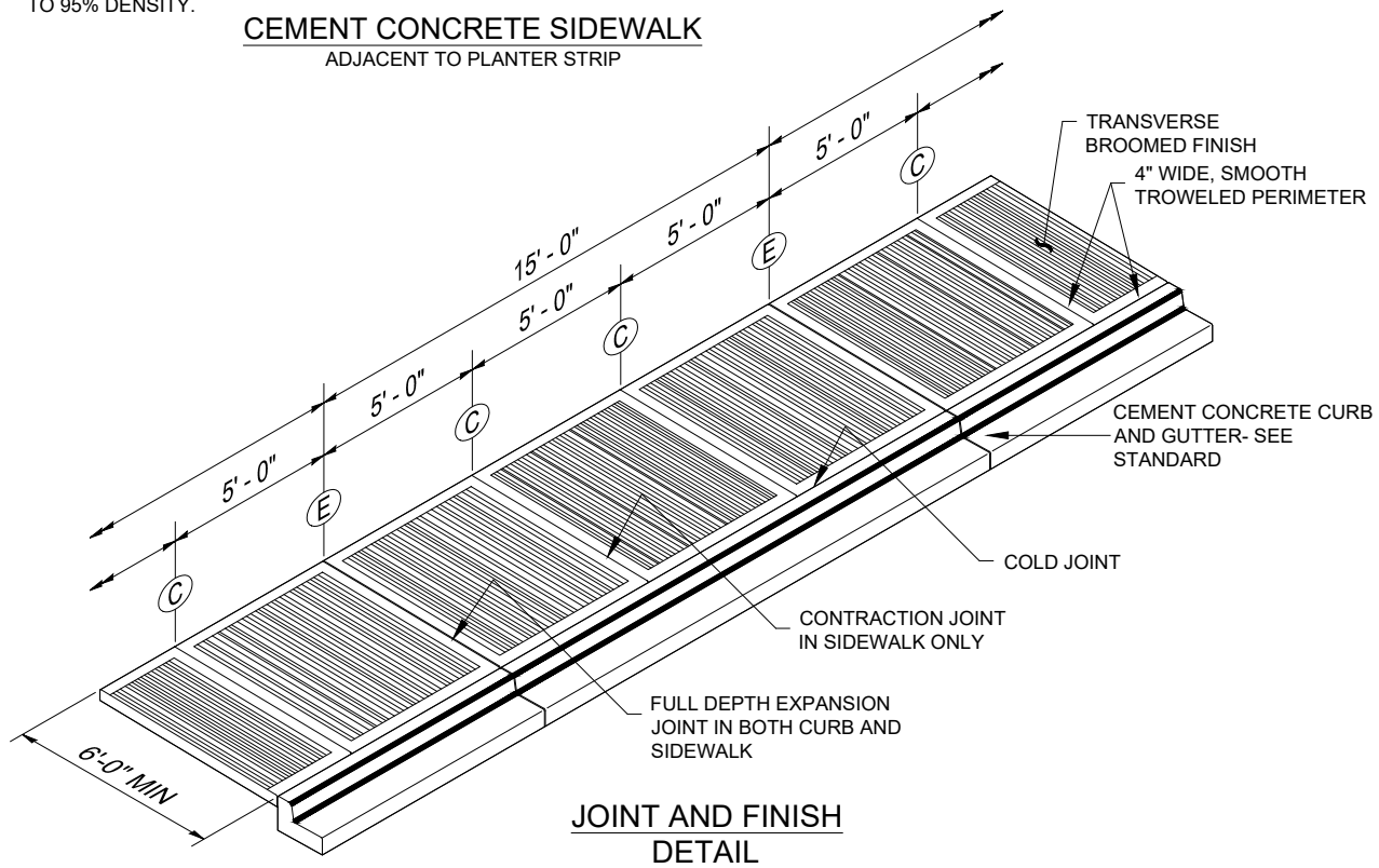
(E) EXPANSION JOINT
