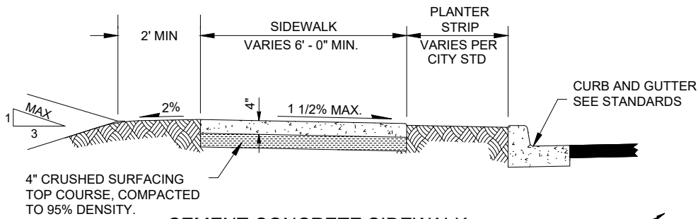
CEMENT CONCRETE SIDEWALK ADJACENT TO PLANTER STRIP
