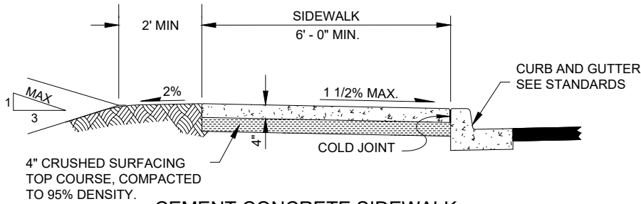
CEMENT CONCRETE SIDEWALK ADJACENT TO CURB
