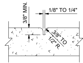
(C) CONTRACTION JOINT
