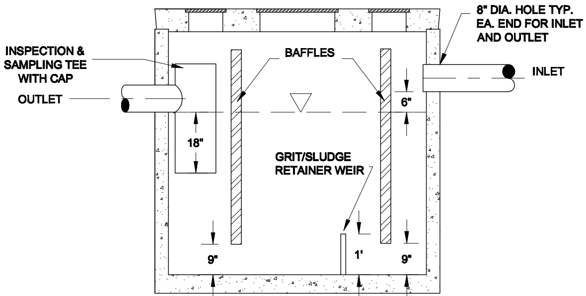
ELEVATION NTS
