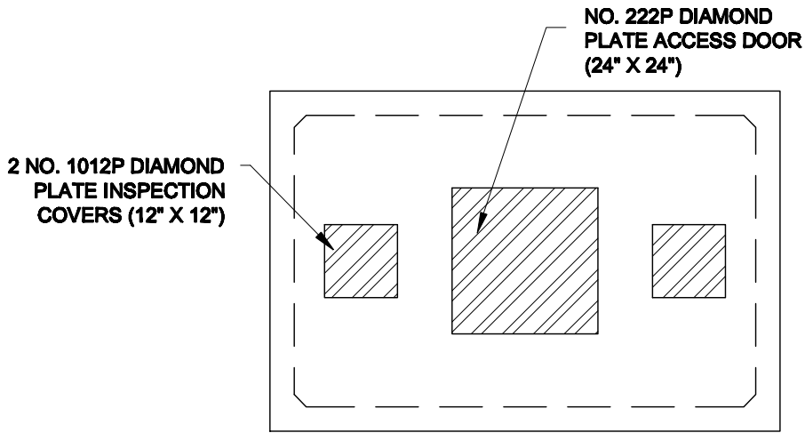
PLAN NTS
