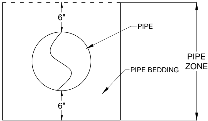
FLEXIBLE PIPE
