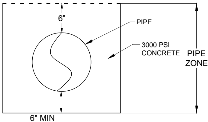
CONCRETE ENCASEMENT
