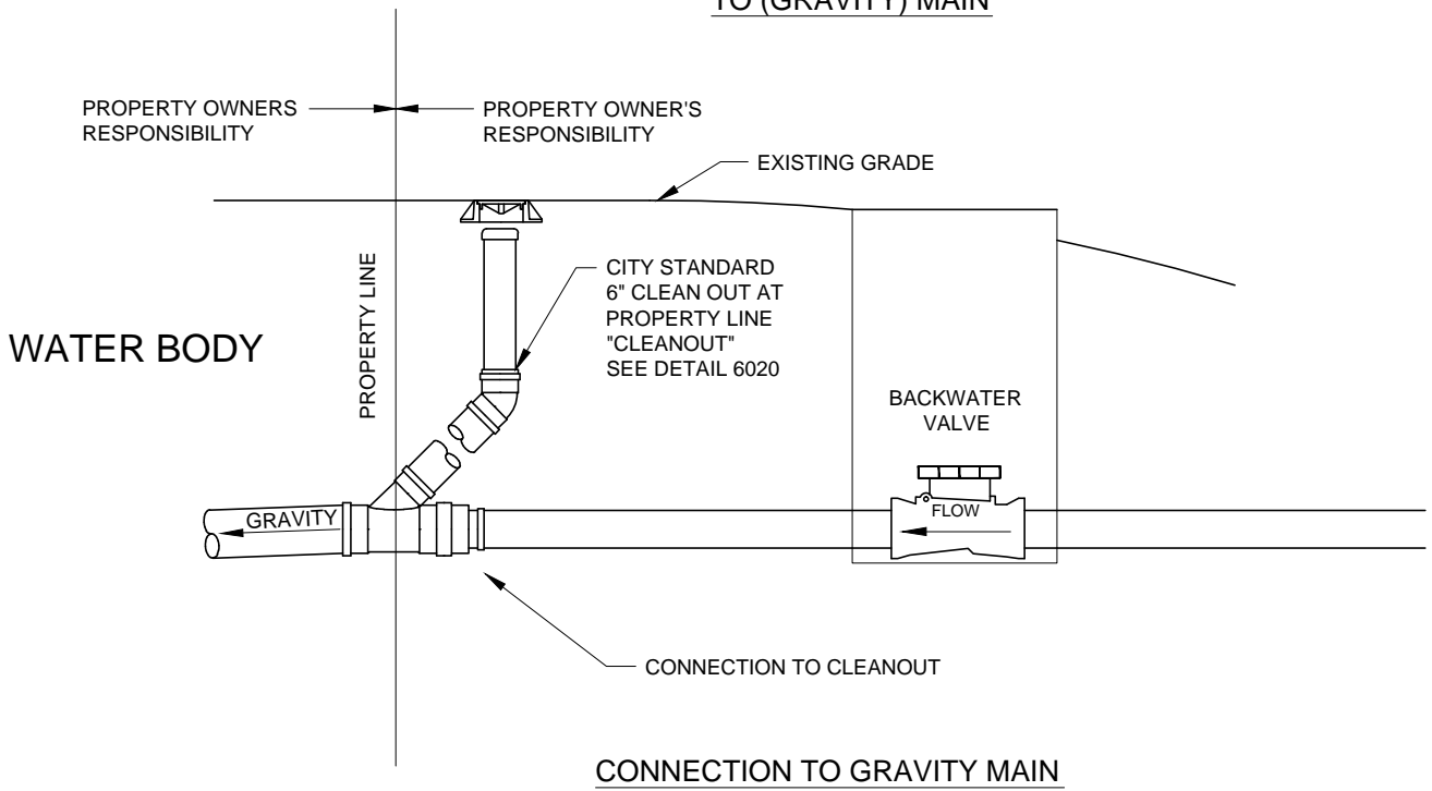
TYPICAL SIDE SEWER CONNECTION TO (GRAVITY) MAIN
