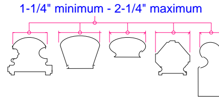
Typical Noncircular Handrail Shapes
