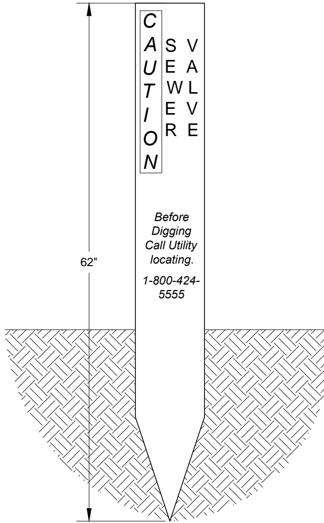
FRONT VIEW
