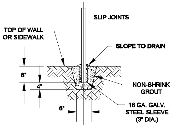
DETAIL A @ POST
