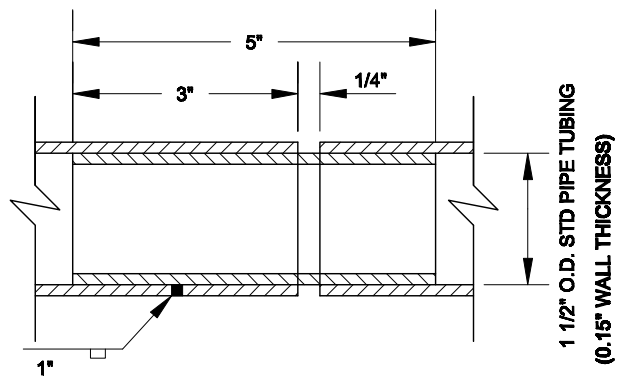
DETAIL B SLIP JOINT DETAIL
